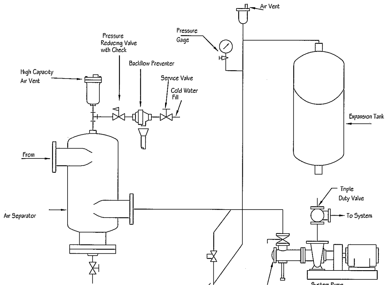
TANQUE DE EXPANSION VERTICAL ESCALA: 5/8"
